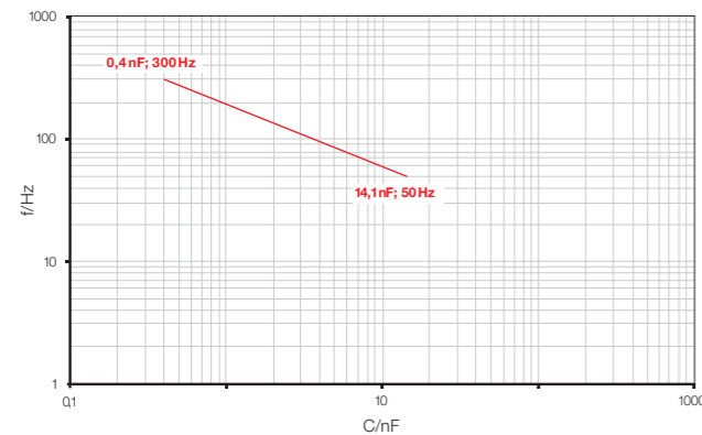
Fig. 4 Test frequency depending on total load capacitance (example WRVG 1.5/680 G)
