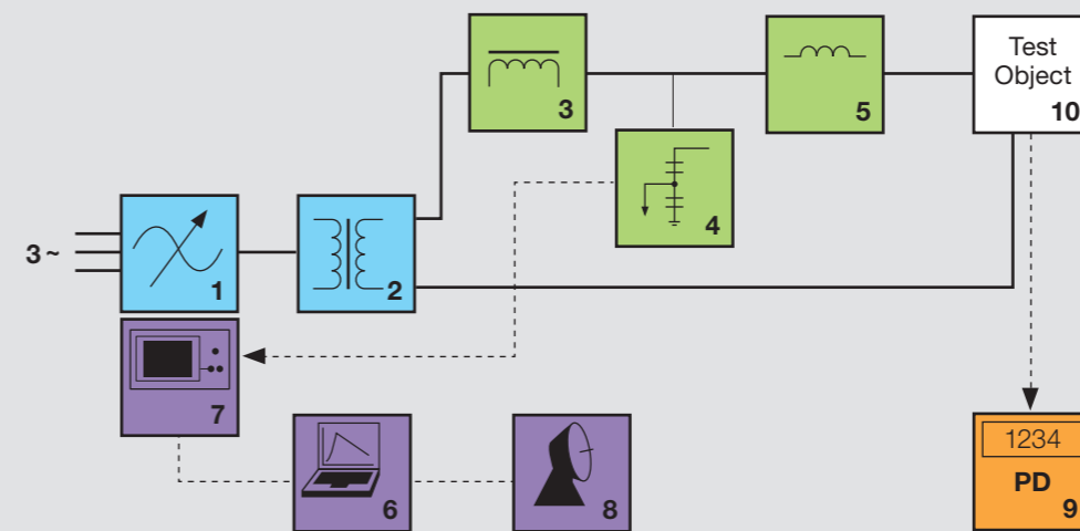
Fig. 3 Block diagram of AC resonant test system for on-site testing of GIS/GIL
